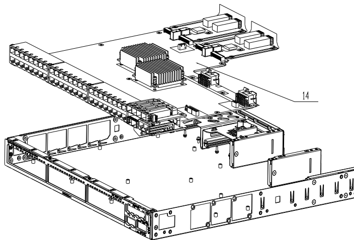
Figure 5 Remove PCB 14
