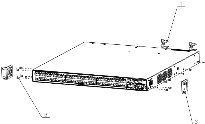
Figure 1 Unscrew the Power Cable Holder 1 and screw 2
