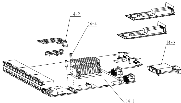
Figure 6 Treatments to PCB 14
