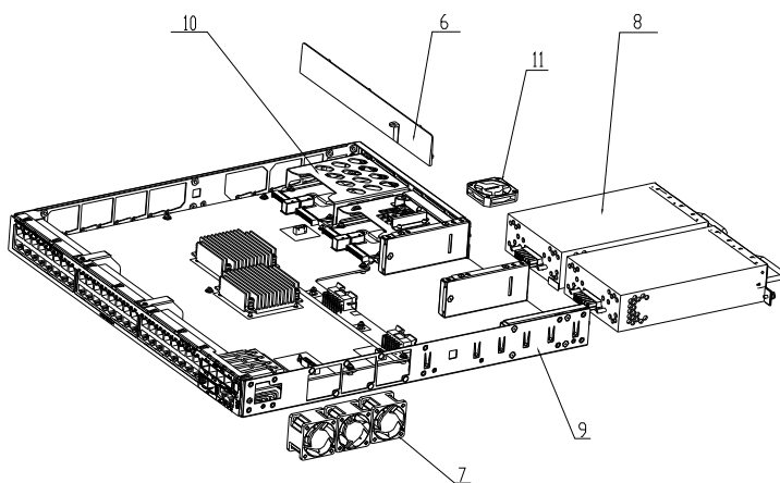
Figure 3 Treatments to the product(I)
