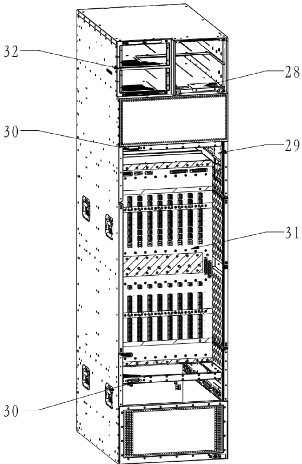
Figure 4 Remove the backboard (rear view)
