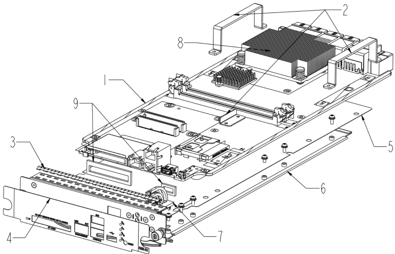
Figure 1 Explode View of the Front Panel
