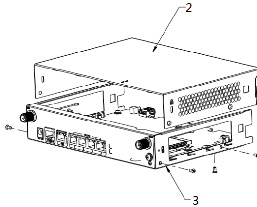
Figure 2 Remove part 2
