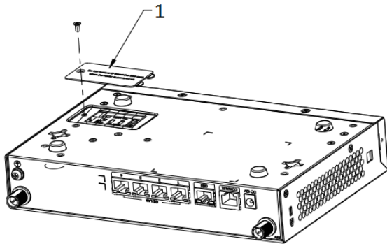
Figure 1 Remove part 1
