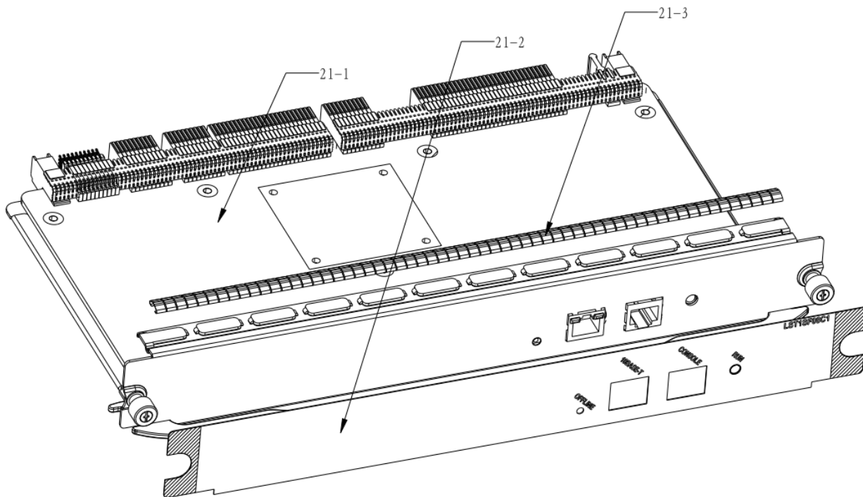
Figure 14 Treatments to panel 21
