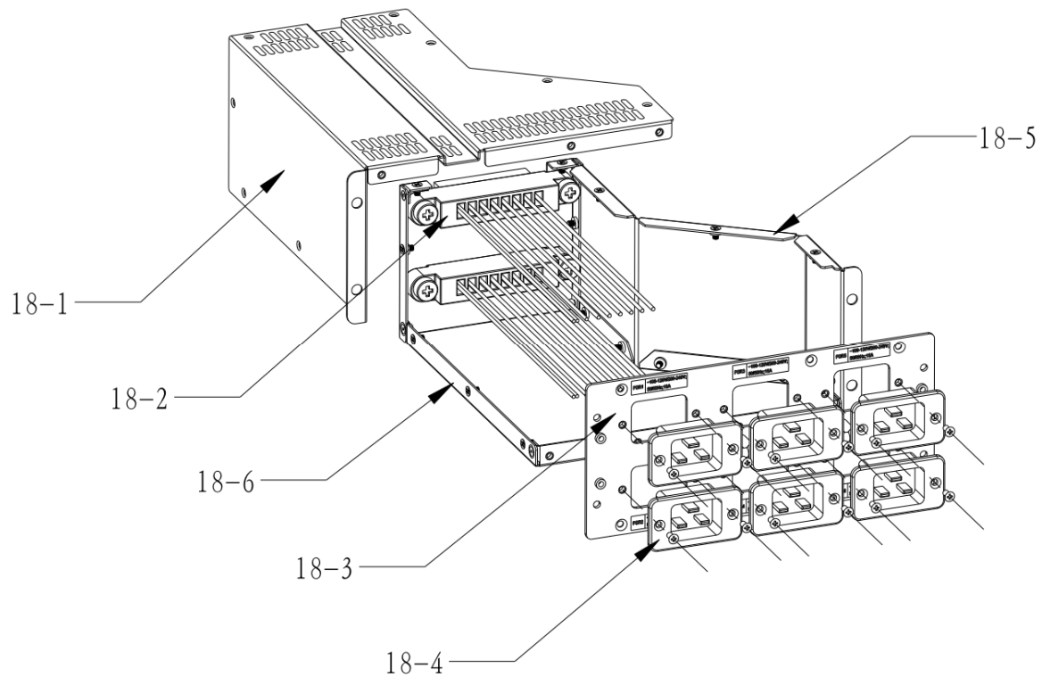
Figure 12 Treatments to PEM 18
