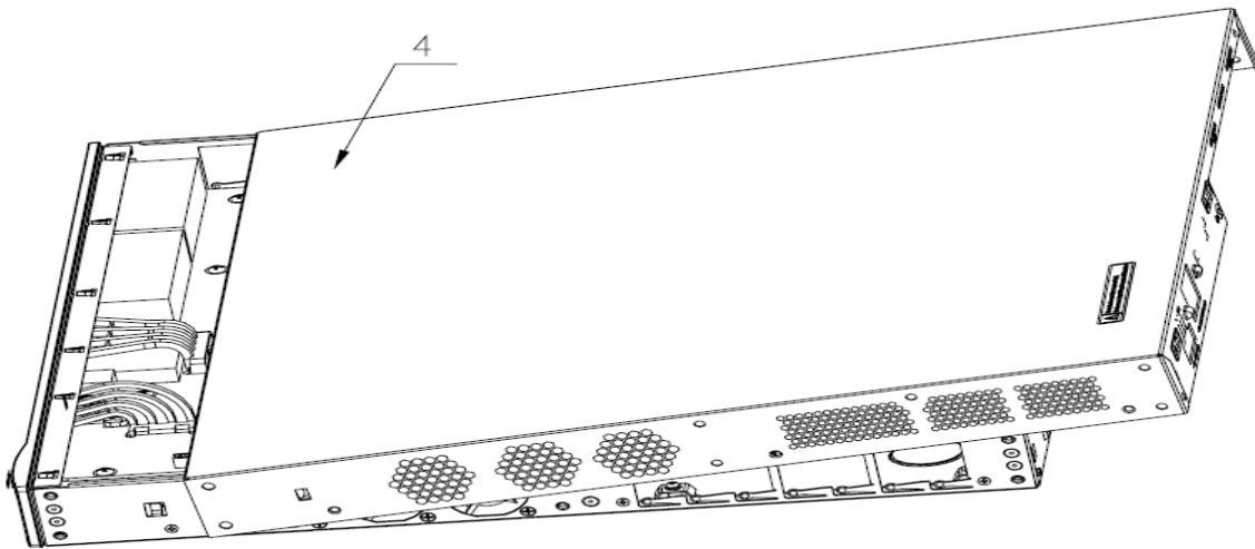
Figure 3 Remove cover
