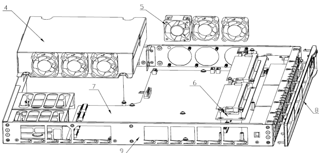
Figure 4 Treatments to the product (remove cover)
