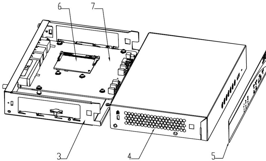
Figure 2 Treatments to the product
