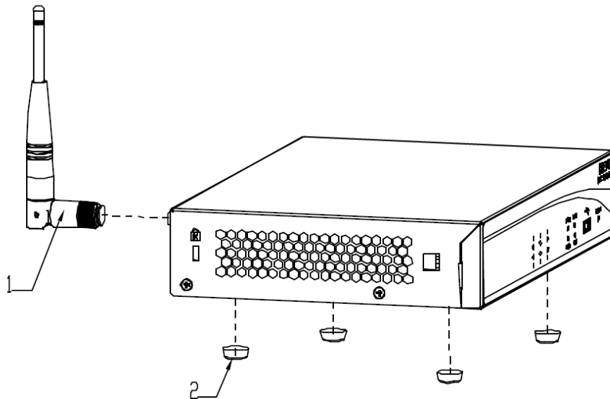
Figure 1 Remove antenna and plastic foot
