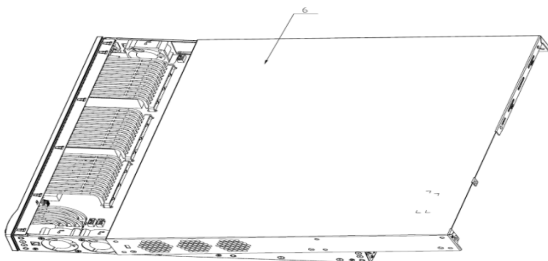
Figure 3 Remove cover
