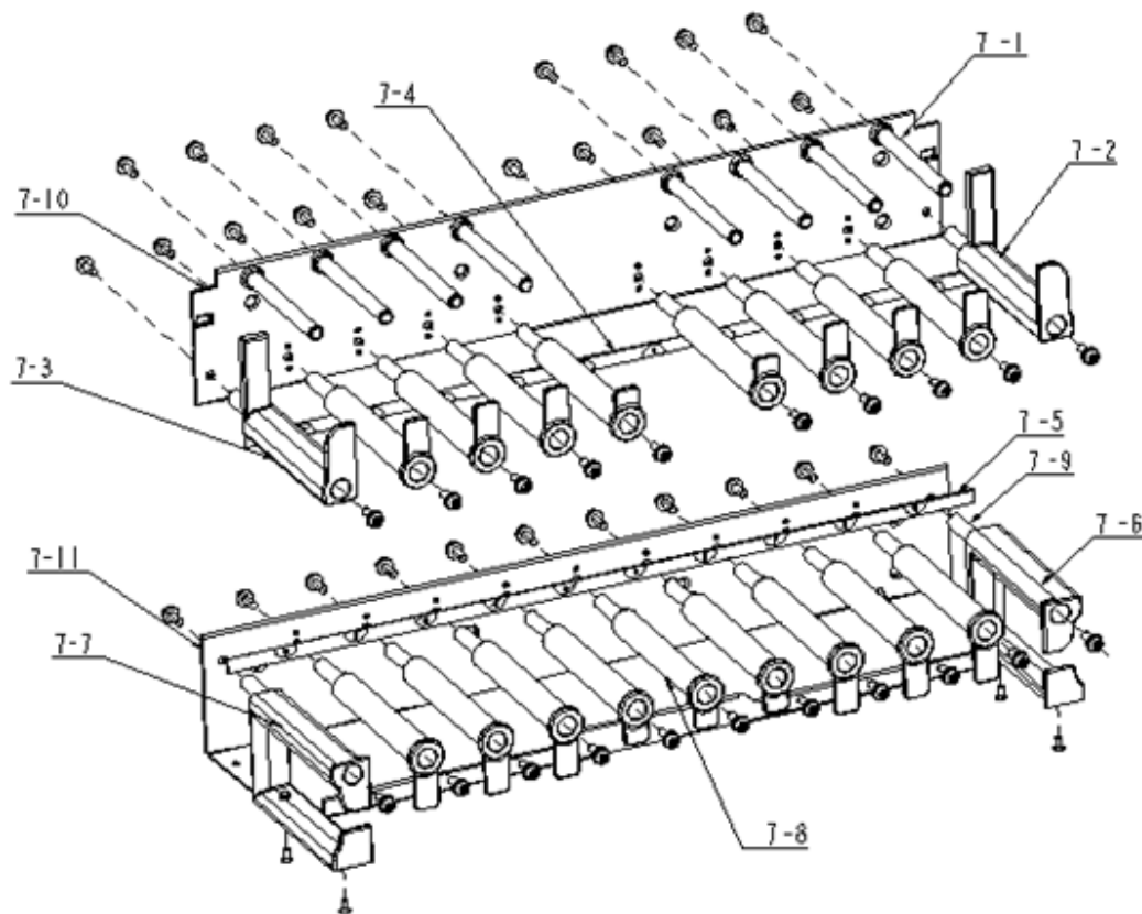
Figure 6 Treatments to wire channel 7
