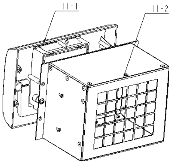
Figure 11 Treatments to blank power module panel 11
