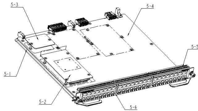
Figure 8 Treatments to front panel 5
