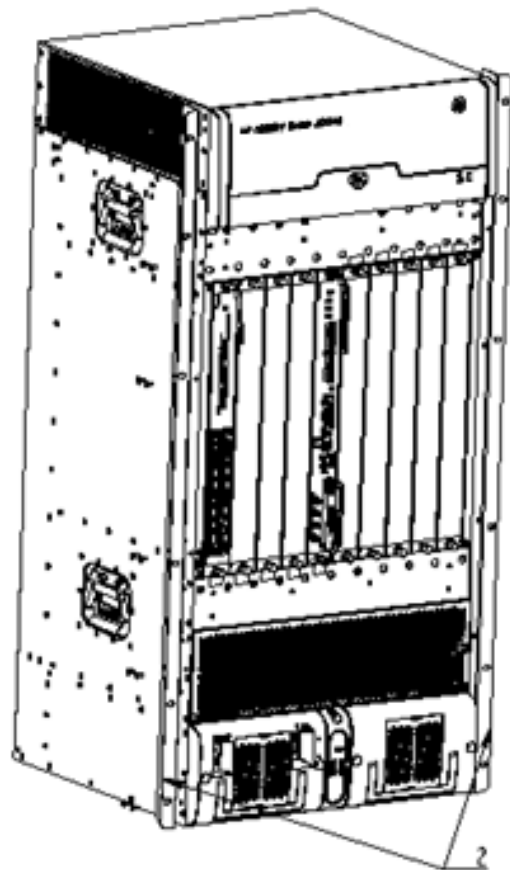
Figure 2 Remove mounting angle
