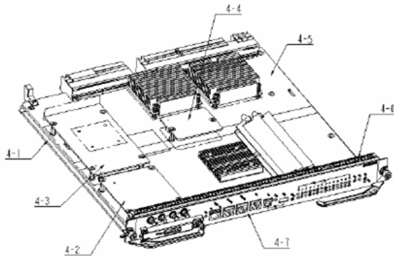
Figure 7 Treatments to front panel 4
