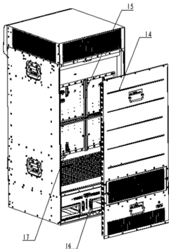
Figure 4 Treatments to the product (rear view)
