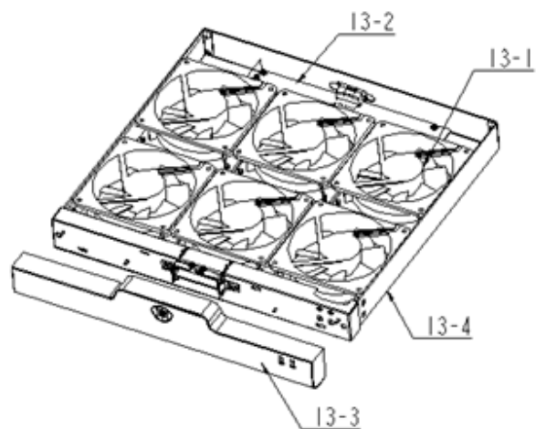
Figure 12 Treatments to fan frame 13
