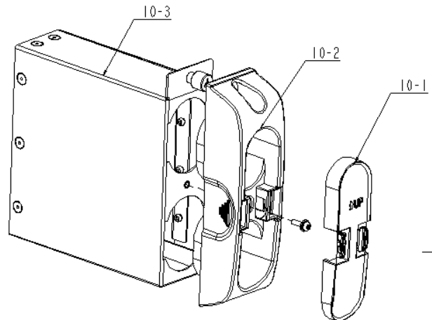
Figure 10 Treatments to blank poe module panel 10
