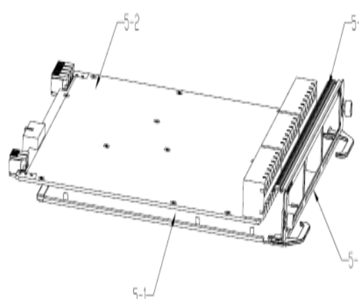
Figure 4 Treatments to front panel 5
