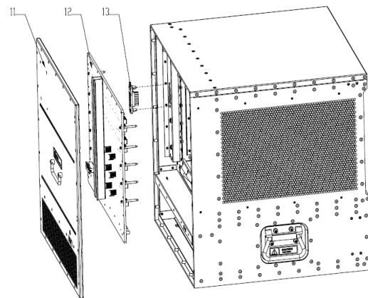
Figure 2 Rear of Quidway S7803
