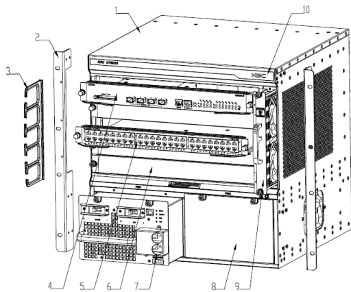
Figure 1 Front of Quidway S7803
