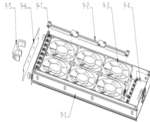
Figure 6 Treatments to fan module frame 9
