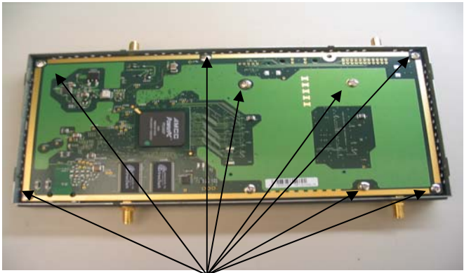
Fig. II – Open these screws to remove PCB from chassis and radio shields
